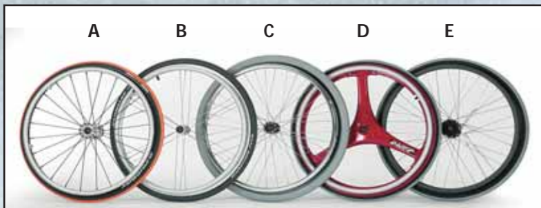
Ruote posteriori: (A) Spinergy, (B) Star 6x3, (C) 36 raggi mozzo piccolo, (D) Racer disponibili nei colori: rosso, blu, grigio e nero, (E) 36 raggi mozzo grande. Rear wheels: (A) Spinergy, (B) Star 6x3, (C) 36 spokes-small hub, (D) Racer available on the following colours: red, blue grey and black, (E) 36 spokes-big hub.
