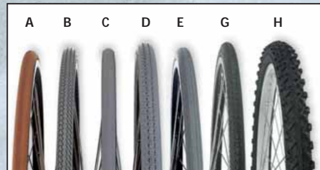
Coperture ruote grandi: (A) tubolare, (B) copertura tassellata alta pressione, (C) copertura liscia alta pressione, (D) copertura pneumatica da 1-3/8, (E) copertura piena da 1, (G) copertura Marathon Plus, (H) copertura pneumatica mountain-bike 24"x1.75. Big wheel tyres: (A) tubular, (B) high pressure plugged tyre, (C) high pressure smooth tyre, (D) 1-3/8 pneumatic tyre, (E) 1 solid tyre, (G) Marathon Plus tyre, (H) Mountain-bike 24"x1.75 pneumatic tyre.
